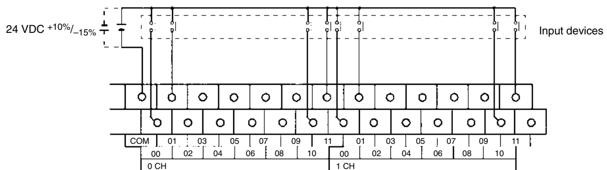
CPM1A-40CDR-□(-V1)/40CDT-□(-V1)/40CDT1-□(-V1)
