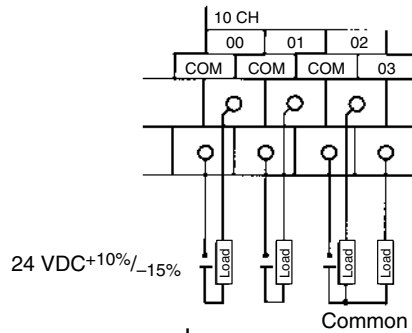
CPM1A-20CDT-□(-V1)/CPM1A-20EDT
