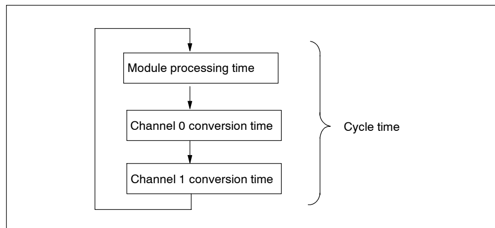
Figure D-6 Cycle time of the analog output module
