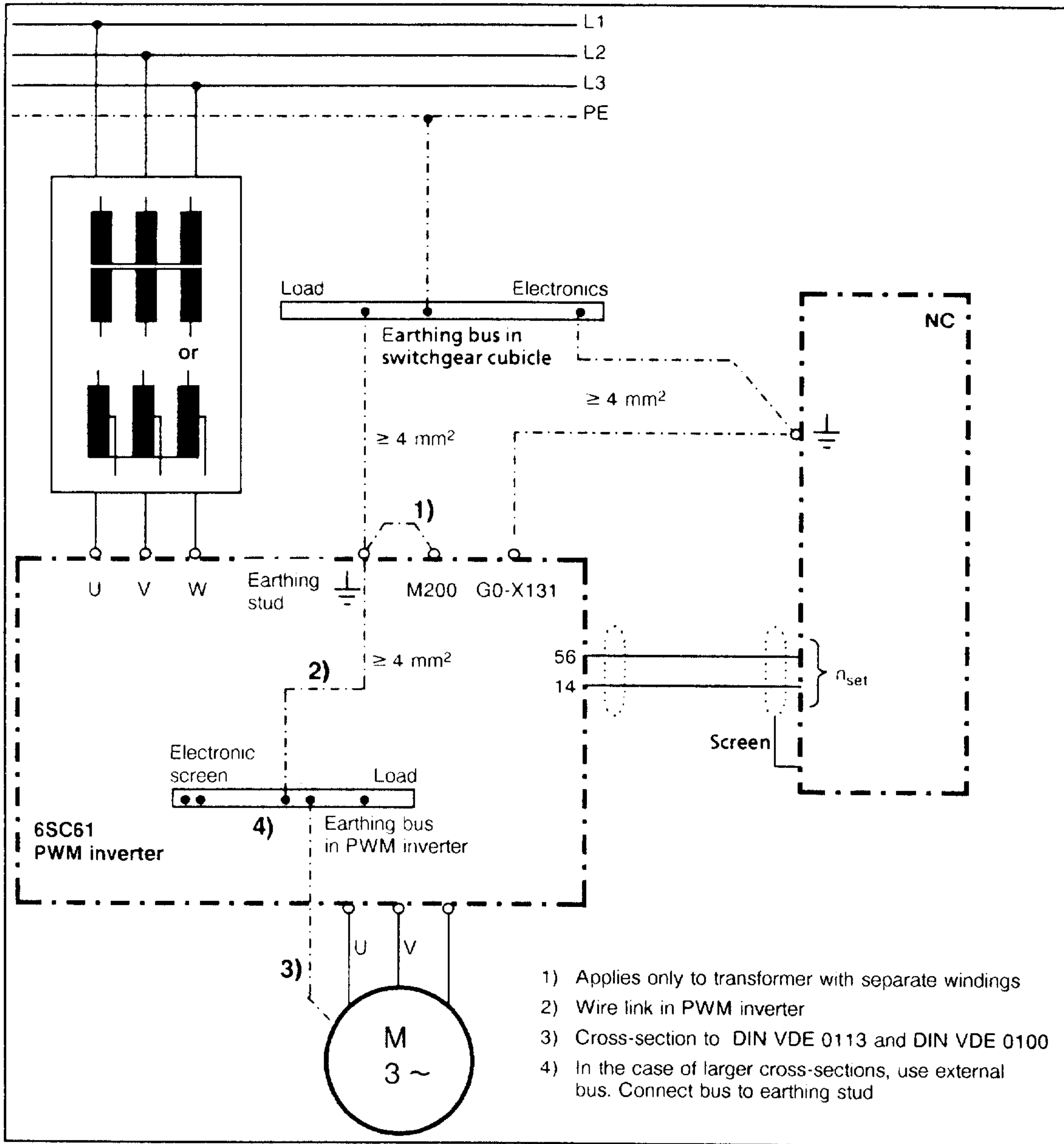
Fig. 2.1 Earthing concept
