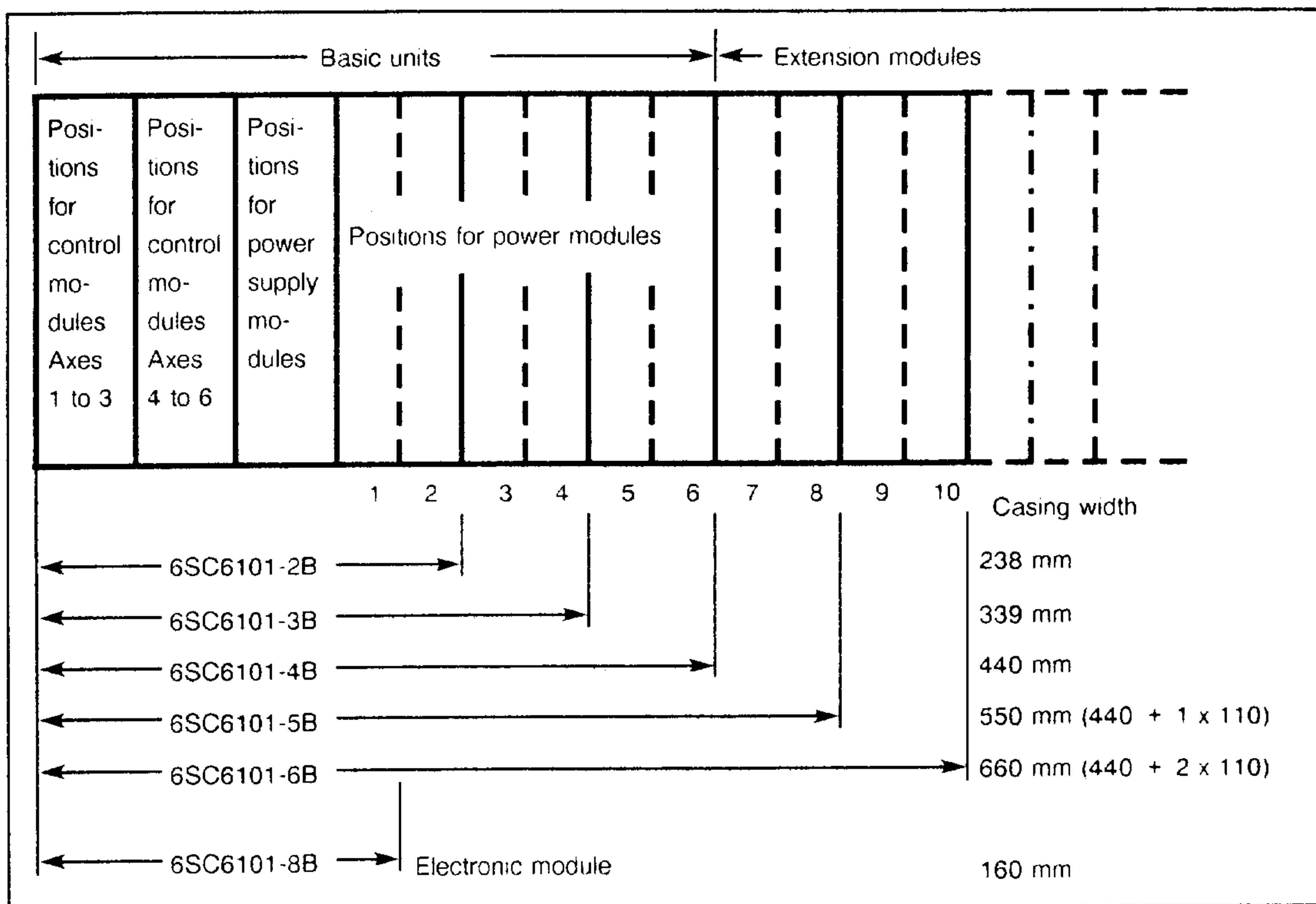
Fig. 1.3 Casing
